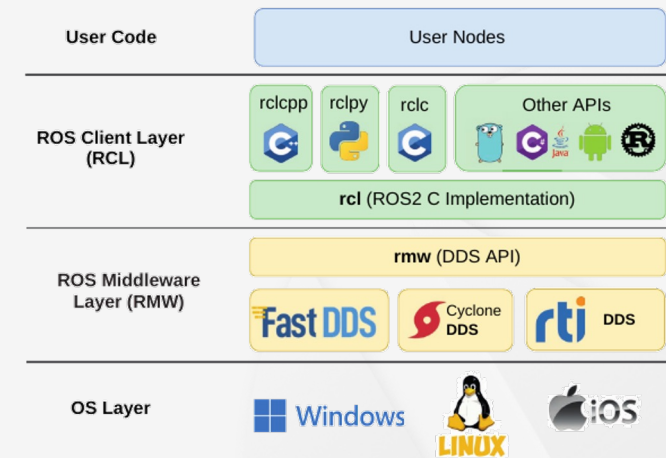
ROS 2 Design
